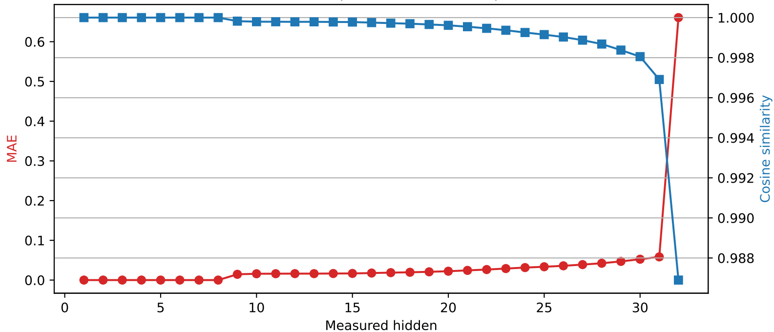
Mistral-7B-Instruct-v0.3 | Quantized layer 8 | float32 \rightarrow int2
