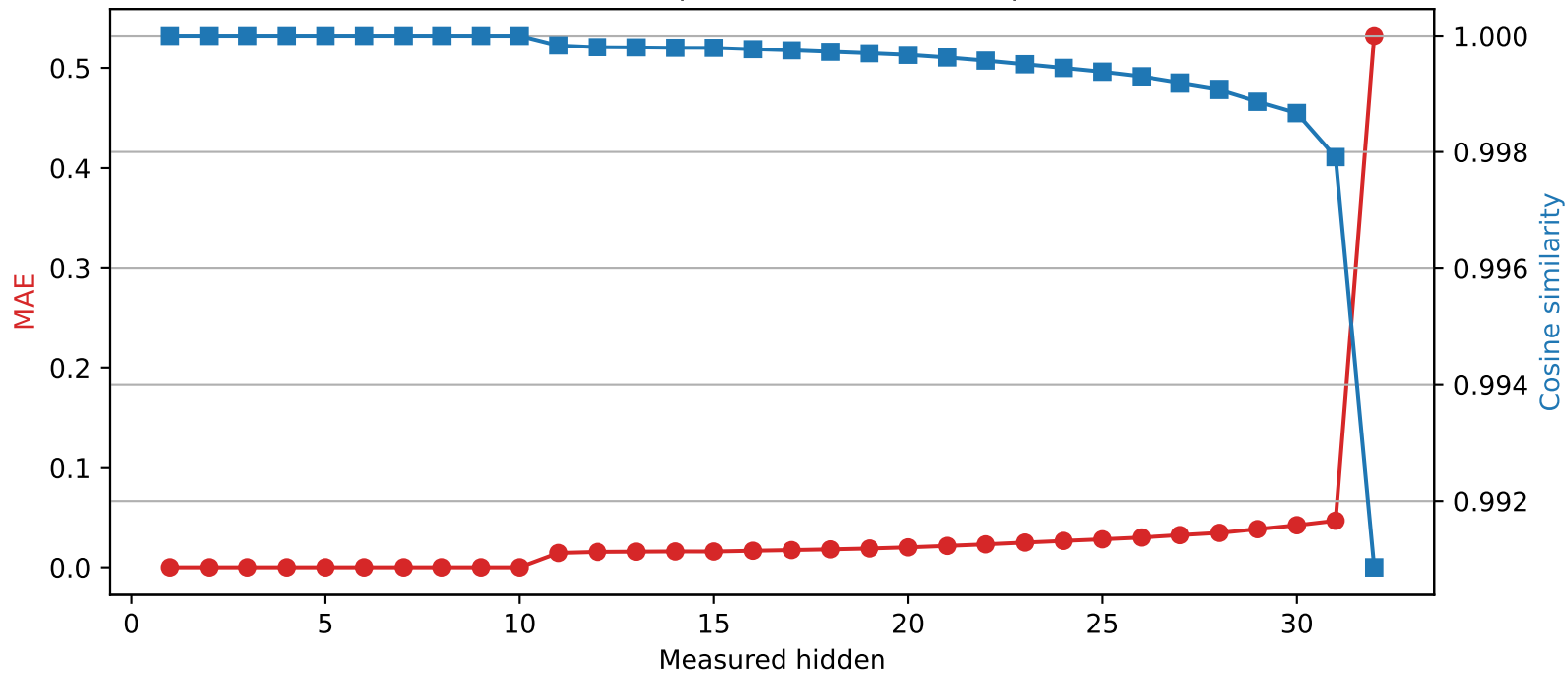
Mistral-7B-Instruct-v0.3 | Quantized layer 10 | float32 → int2
