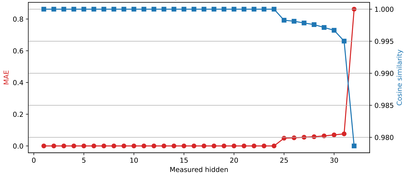
Mistral-7B-Instruct-v0.3 | Quantized layer 24 | float32 → int2
