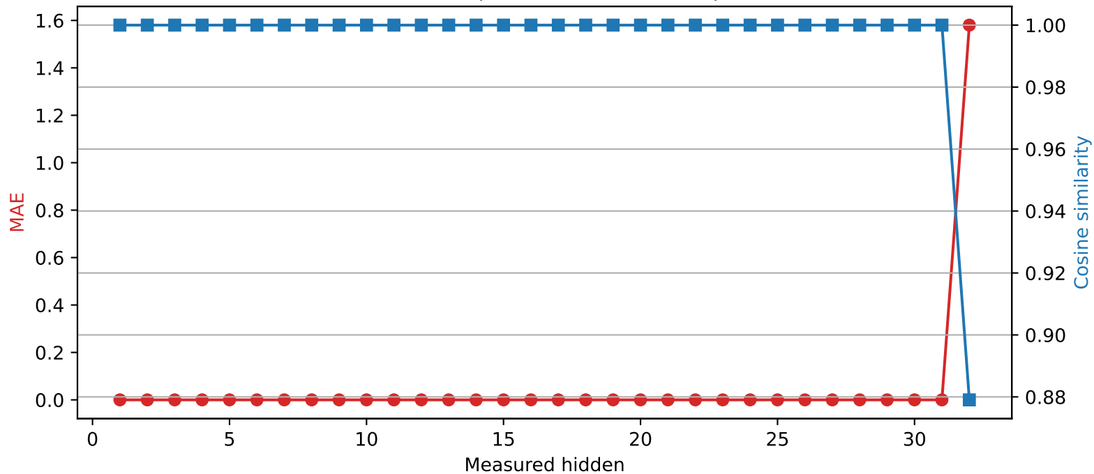
Mistral-7B-Instruct-v0.3 | Quantized layer 31 | float32 \rightarrow int2
