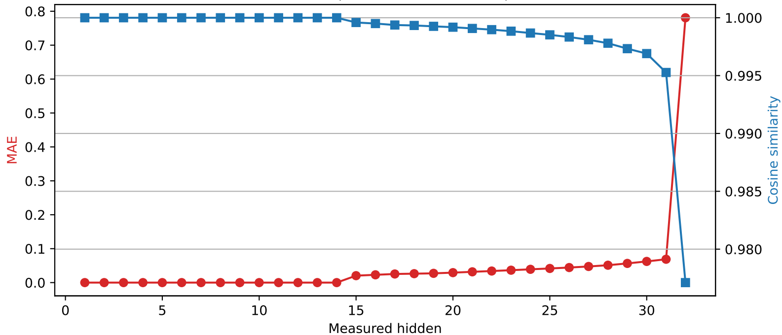
Mistral-7B-Instruct-v0.3 | Quantized layer 14 | float32 → int2
