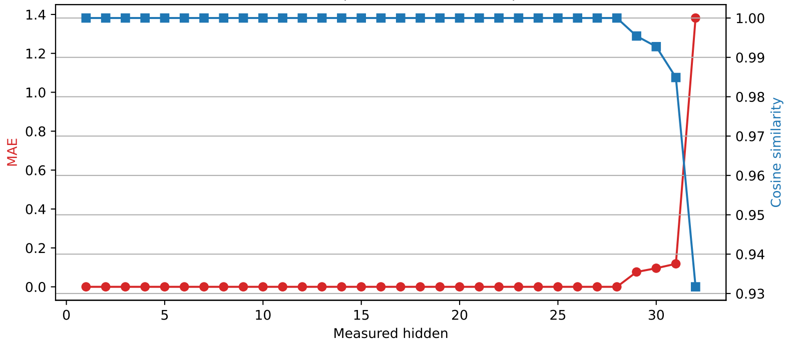
Mistral-7B-Instruct-v0.3 | Quantized layer 28 | float32 → int2
