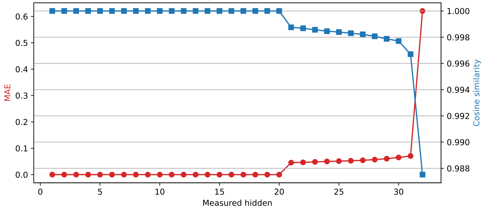
Mistral-7B-Instruct-v0.3 | Quantized layer 20 | float32 → int2
