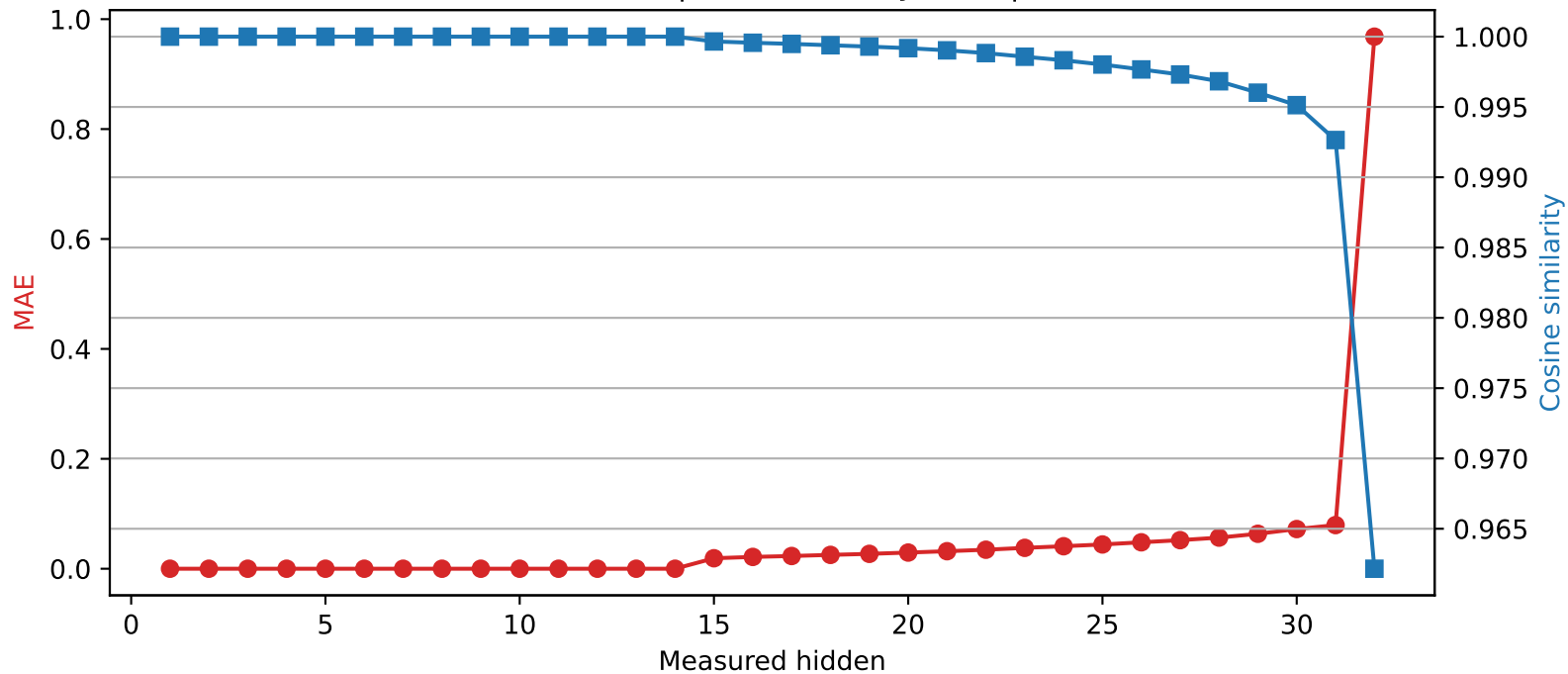
Mistral-7B-Instruct-v0.3 | Quantized layer 14 | float64 → int2
