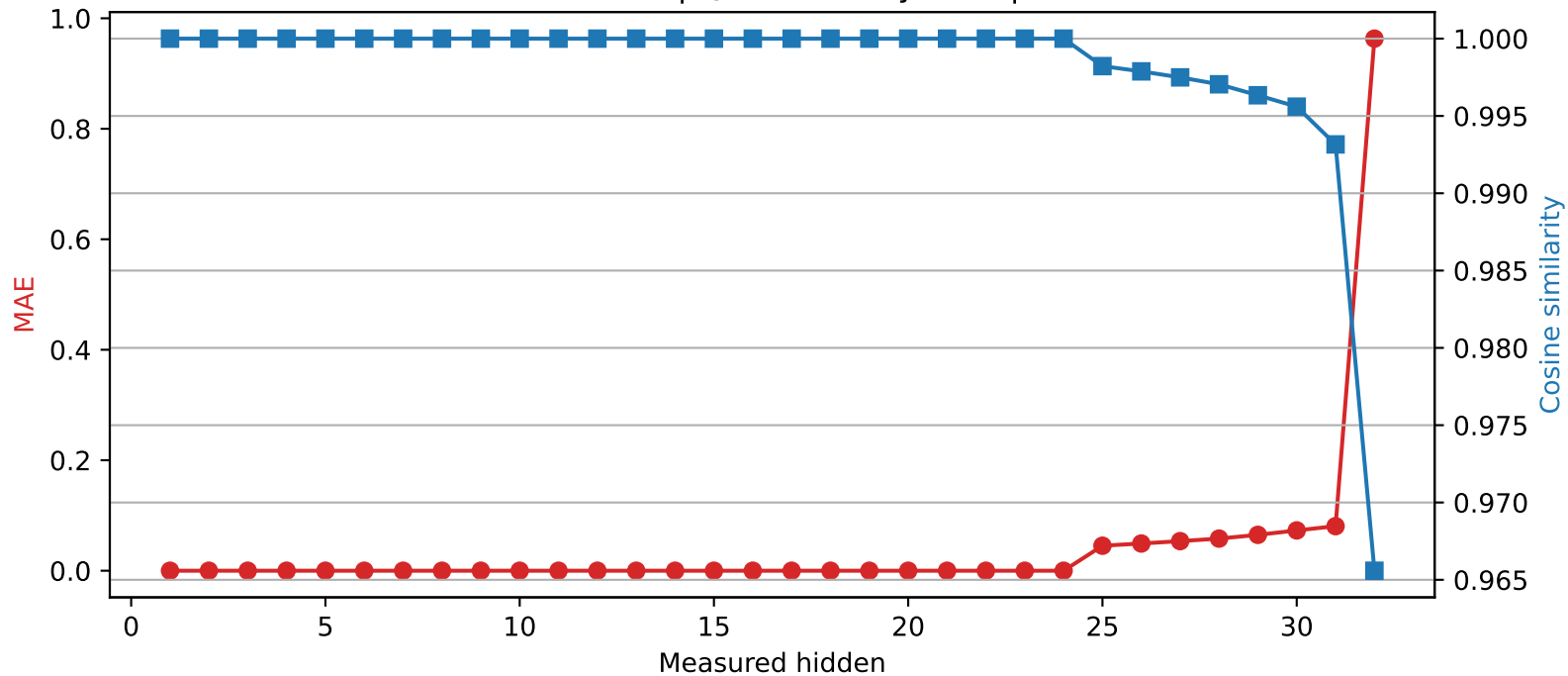
Mistral-7B-Instruct-v0.3 | Quantized layer 24 | float64 → int2
