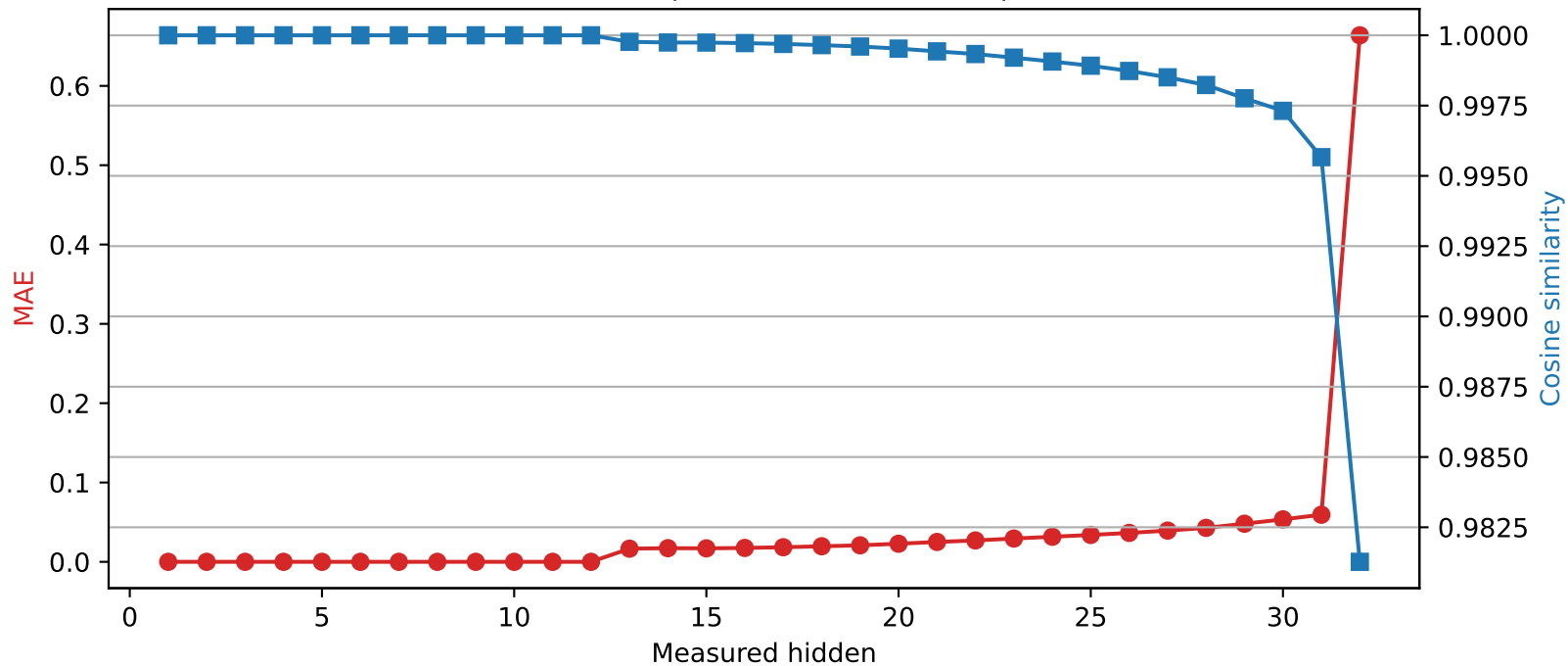
Mistral-7B-Instruct-v0.3 | Quantized layer 12 | float64 → int2
