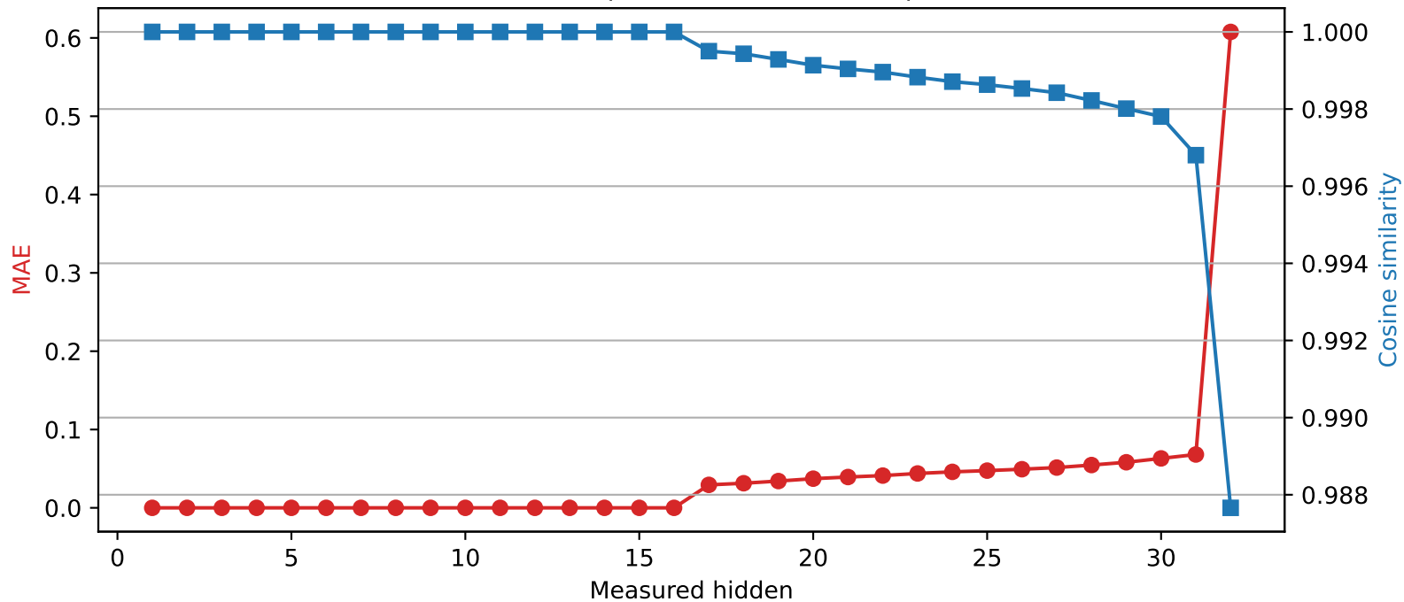
Mistral-7B-Instruct-v0.3 | Quantized layer 16 | float64 → int2
