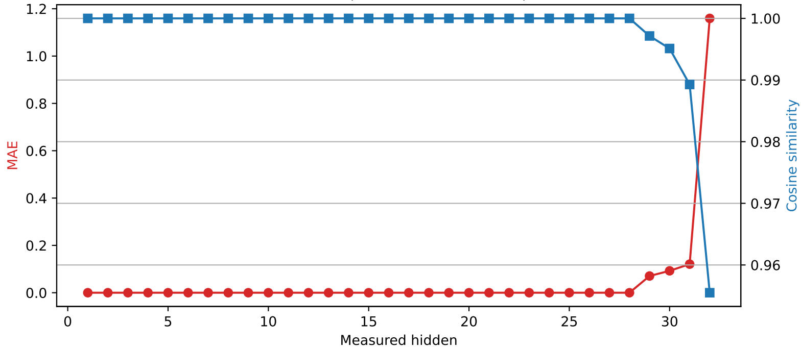
Mistral-7B-Instruct-v0.3 | Quantized layer 28 | float64 → int2
