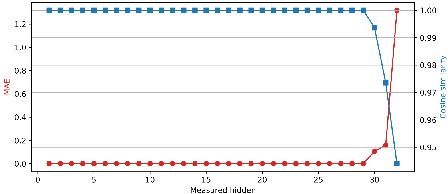
Mistral-7B-Instruct-v0.3 | Quantized layer 29 | float64 → int2
