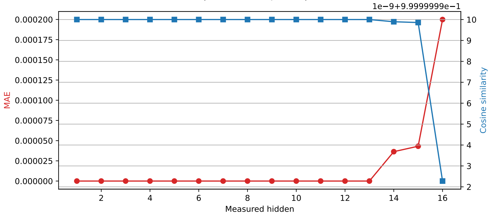
Llama-3.2-1B | Quantized layer 13 | float32 → int16
