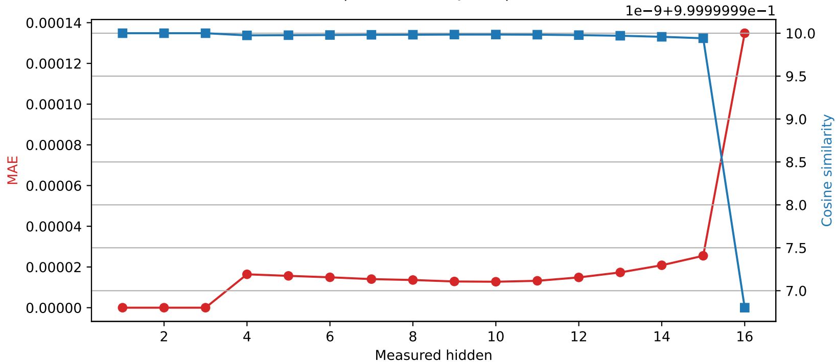
Llama-3.2-1B | Quantized layer 3 | float32 → int16
