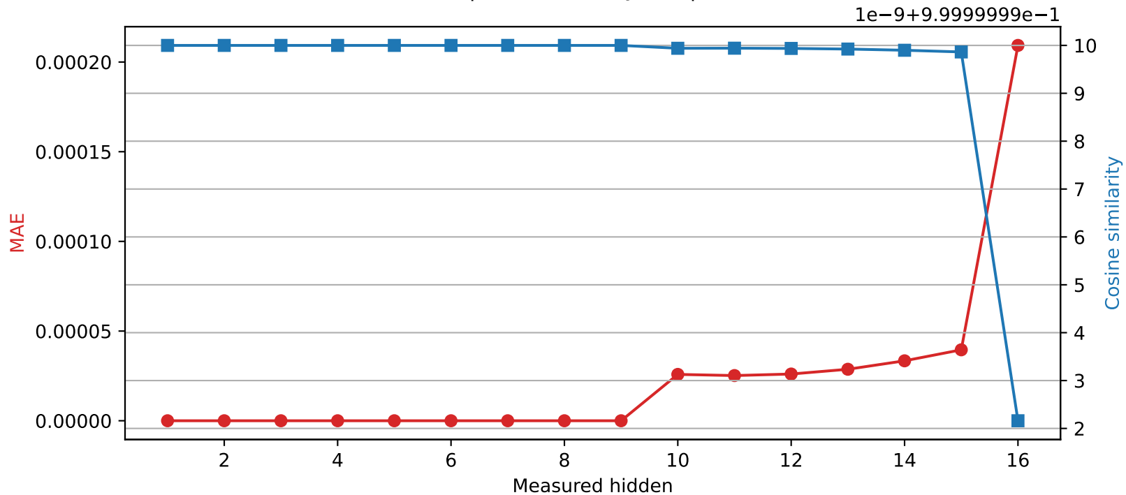
Llama-3.2-1B | Quantized layer 9 | float32 → int16
