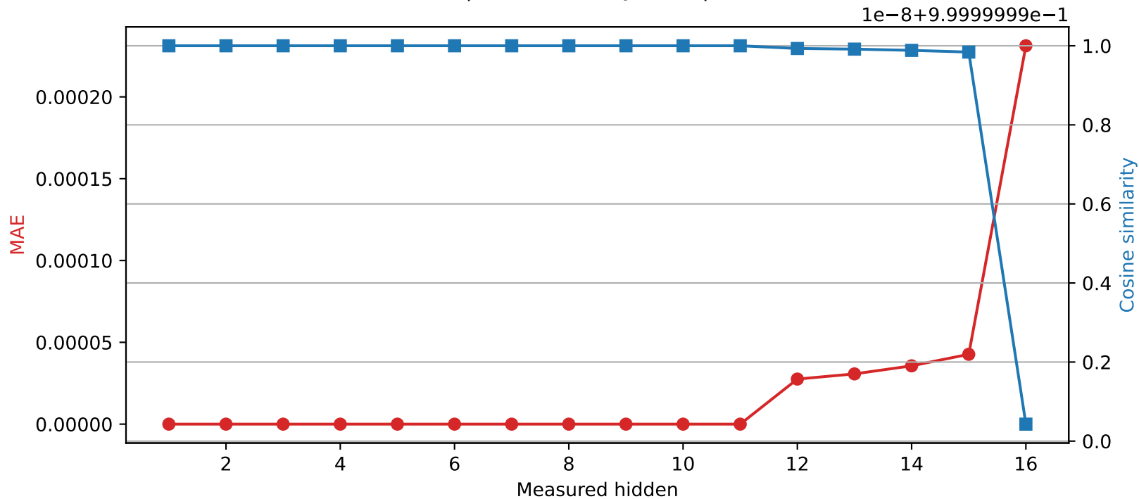
Llama-3.2-1B | Quantized layer 11 | float32 \rightarrow int16
