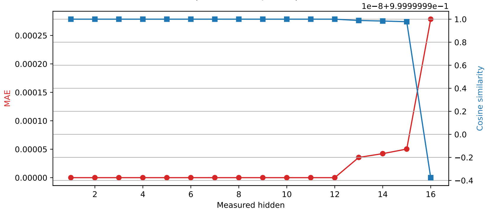
Llama-3.2-1B | Quantized layer 12 | float32 → int16
