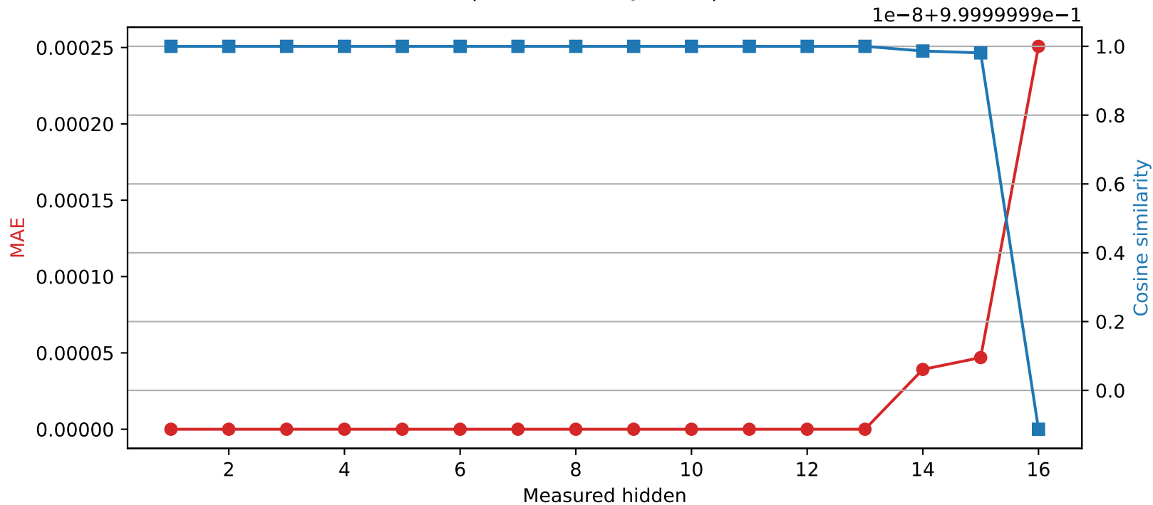
Llama-3.2-1B | Quantized layer 13 | float32 \rightarrow int16
