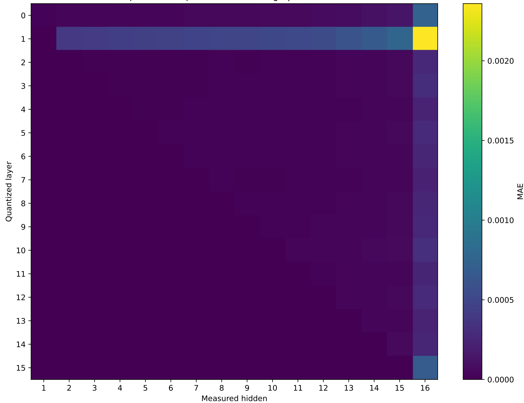
Llama-3.2-1B Prompt 3: MAE representation damage | float32 → int16
