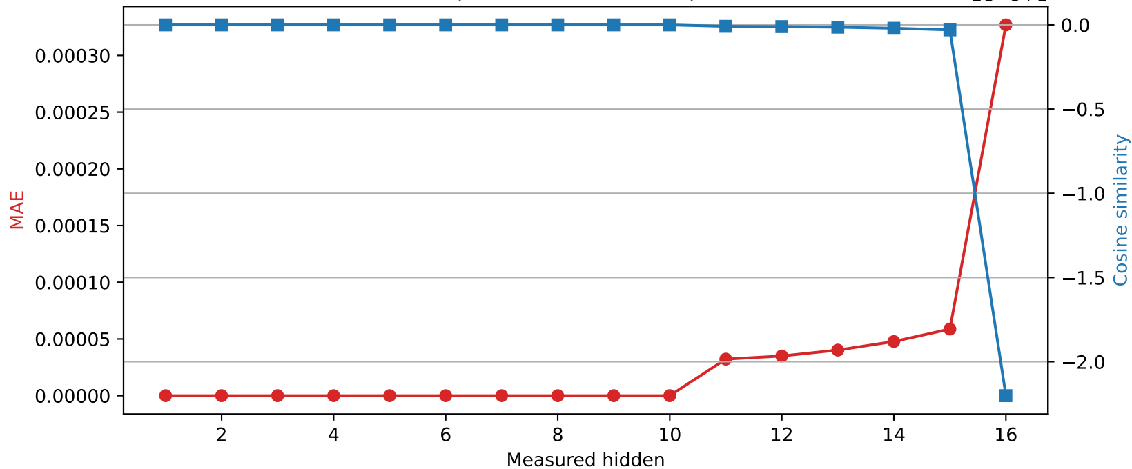
Llama-3.2-1B | Quantized layer 10 | float32 → int16
