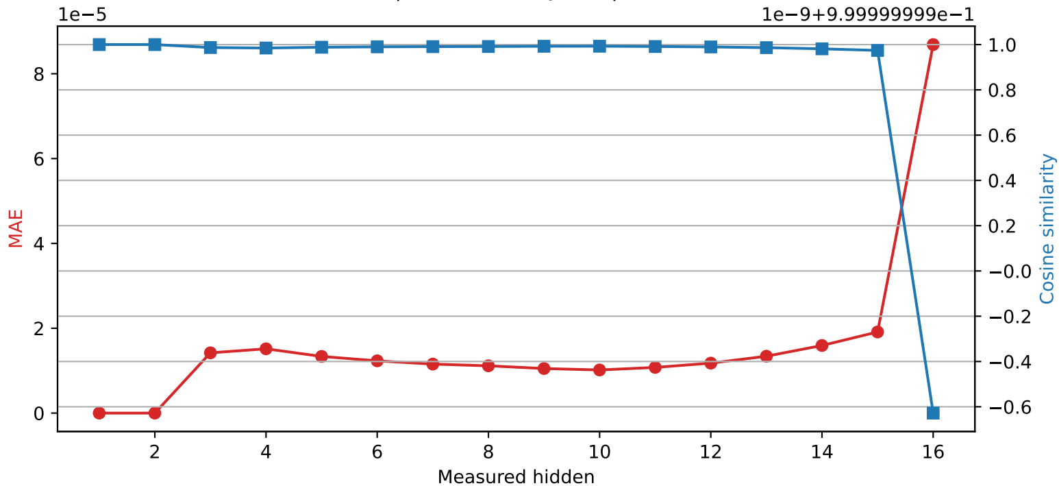
Llama-3.2-1B | Quantized layer 2 | float32 \rightarrow int16
