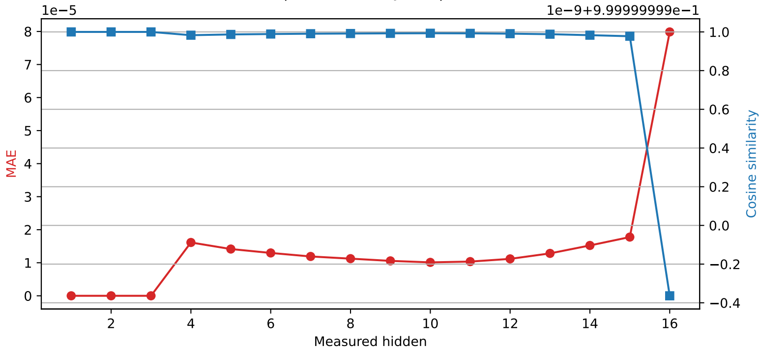
Llama-3.2-1B | Quantized layer 3 | float32 \rightarrow int16
