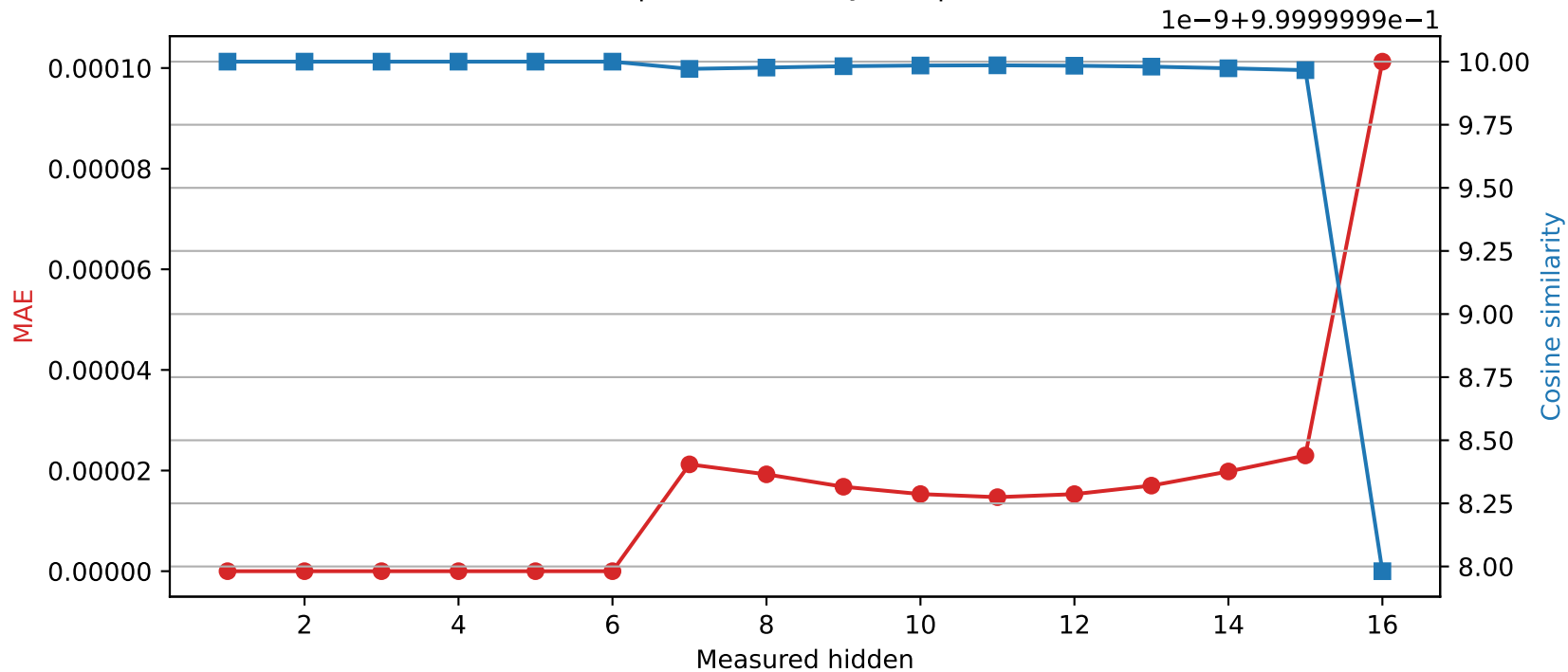
Llama-3.2-1B | Quantized layer 6 | float32 → int16
