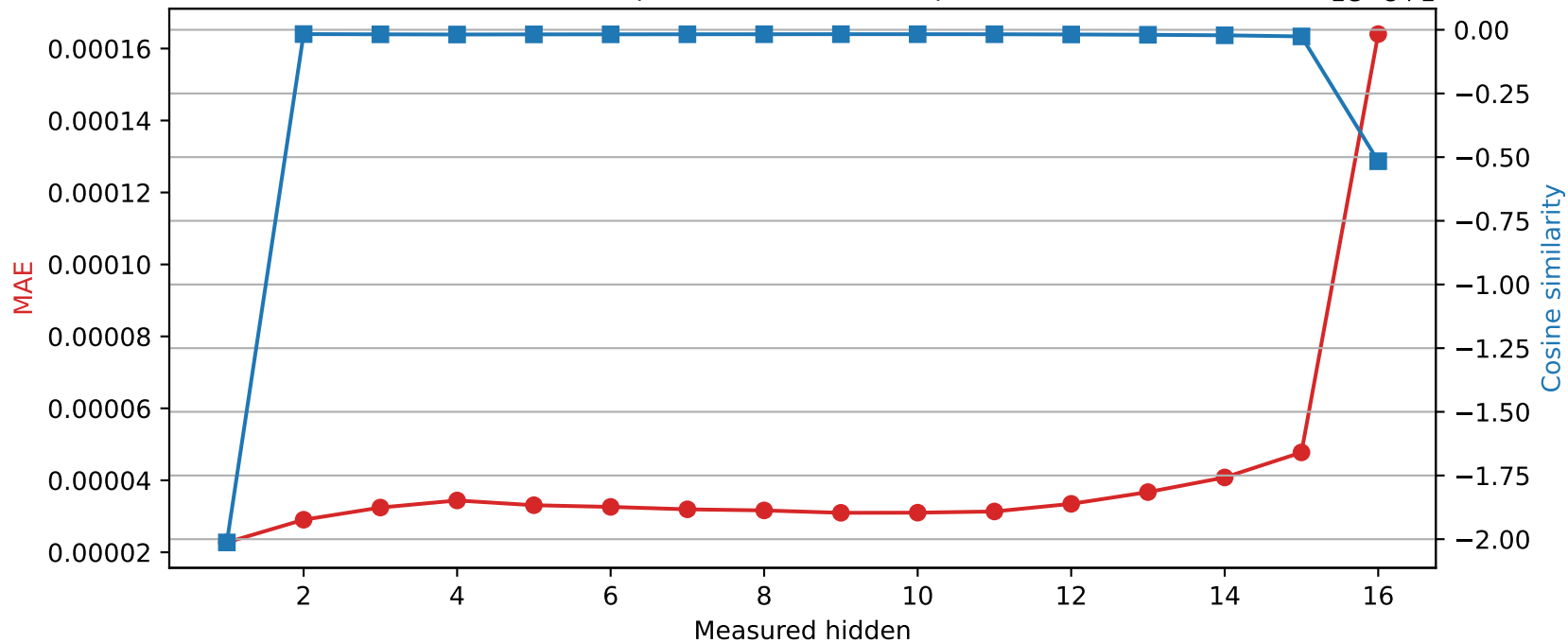
Llama-3.2-1B | Quantized layer 0 | float64 → int16
