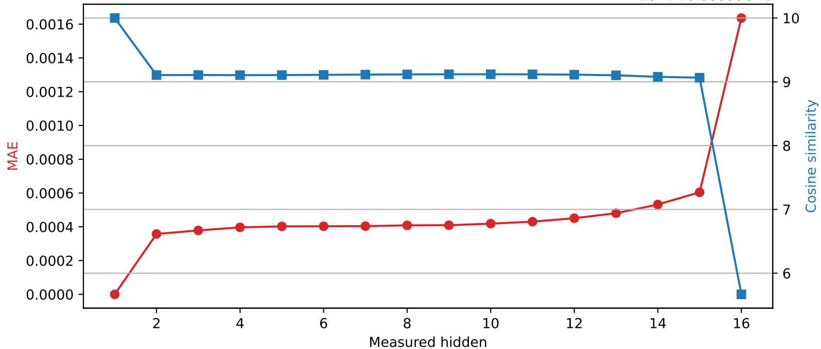
Llama-3.2-1B | Quantized layer 1 | float64 \rightarrow int16 1e-7+9.99999e-1
