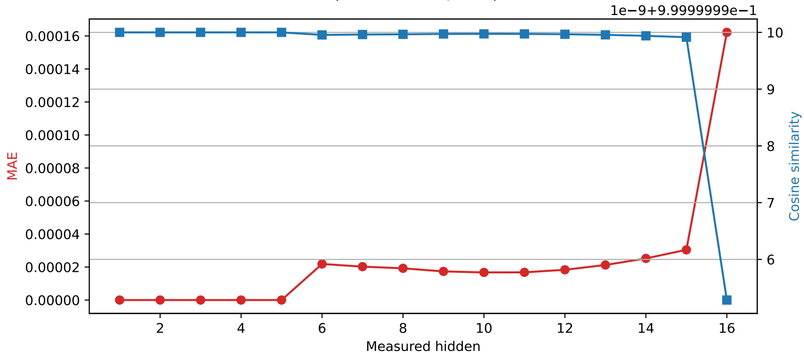
Llama-3.2-1B | Quantized layer 5 | float64 → int16
