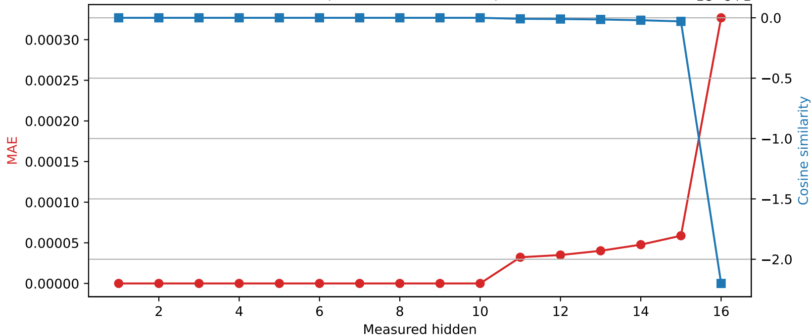
Llama-3.2-1B | Quantized layer 10 | float64 → int16
