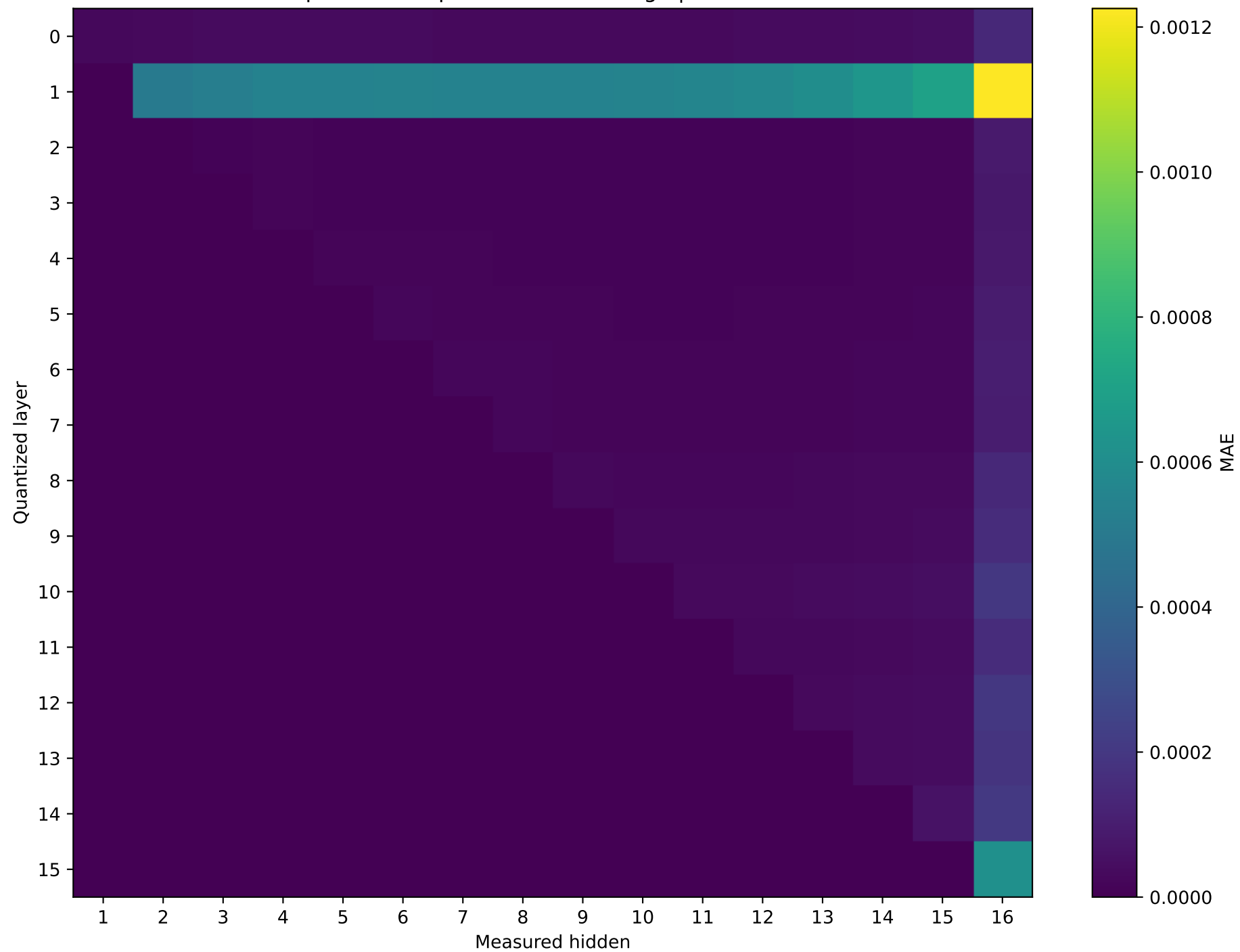
Llama-3.2-1B Prompt 4: MAE representation damage | float64 → int16
