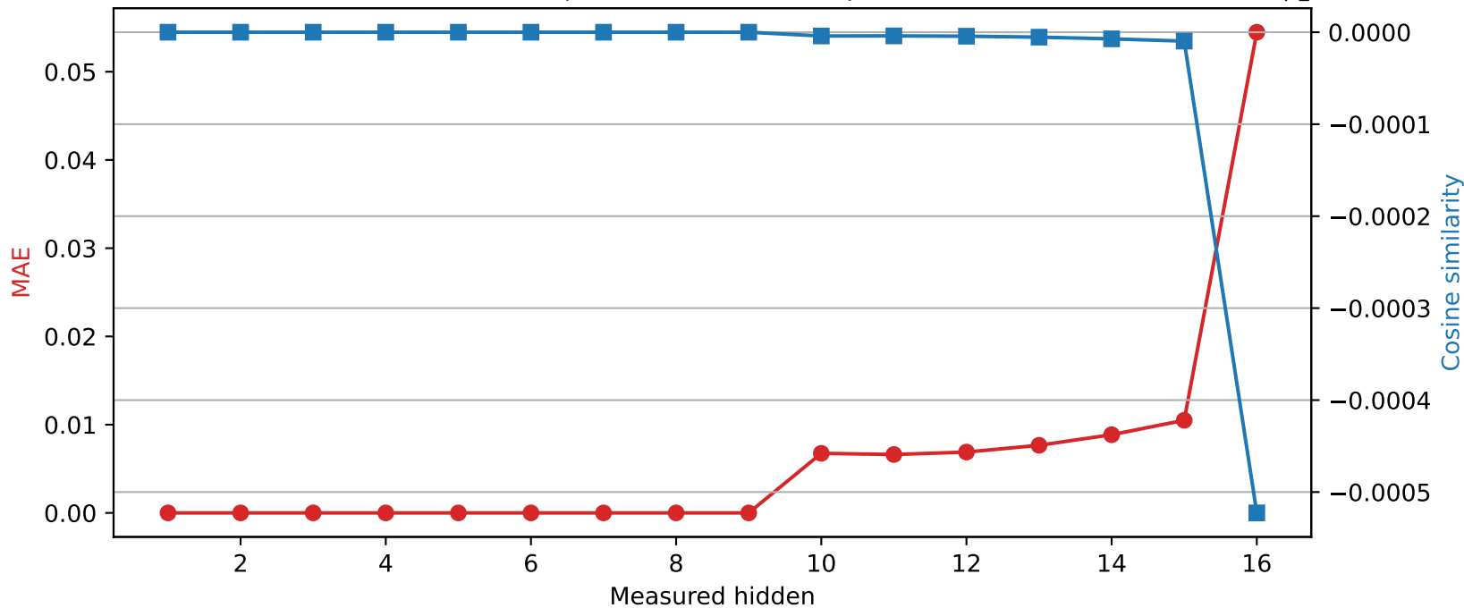
Llama-3.2-1B | Quantized layer 9 | float16 \rightarrow int8
