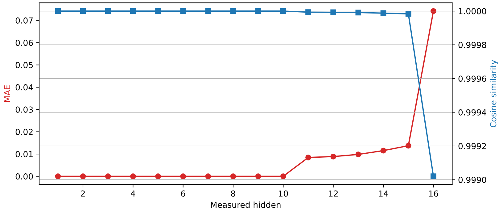
Llama-3.2-1B | Quantized layer 10 | float16 \rightarrow int8
