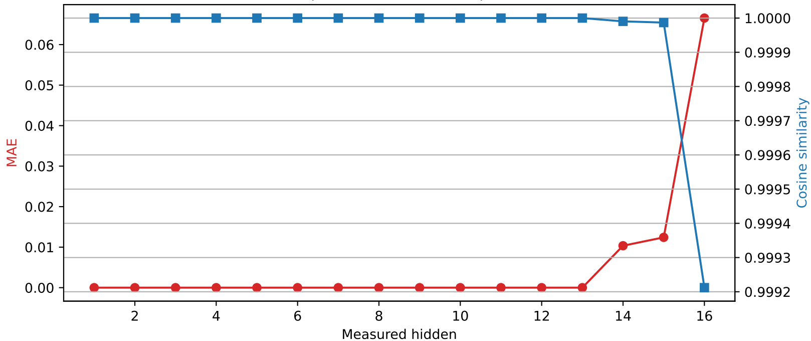
Llama-3.2-1B | Quantized layer 13 | float16 → int8
