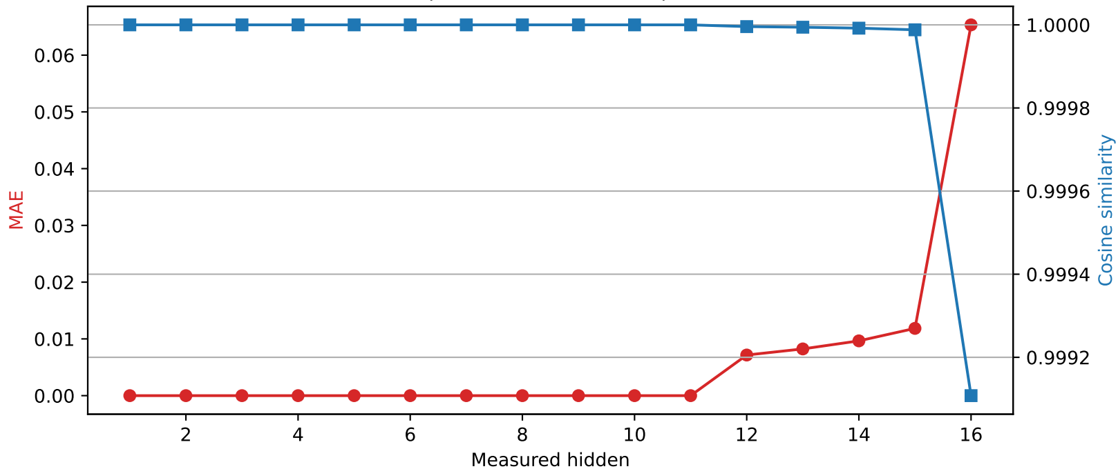
Llama-3.2-1B | Quantized layer 11 | float16 \rightarrow int8
