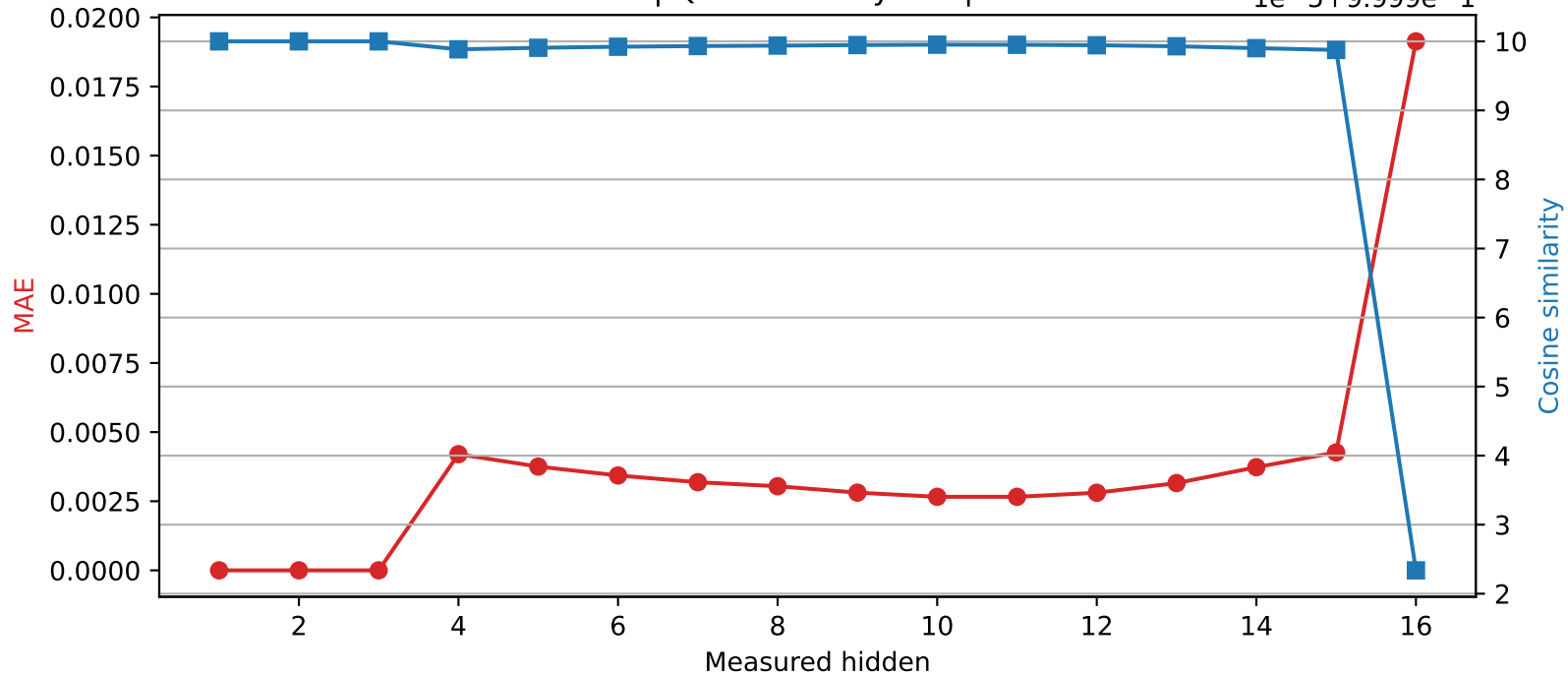
Llama-3.2-1B | Quantized layer 3 | float16 → int8
