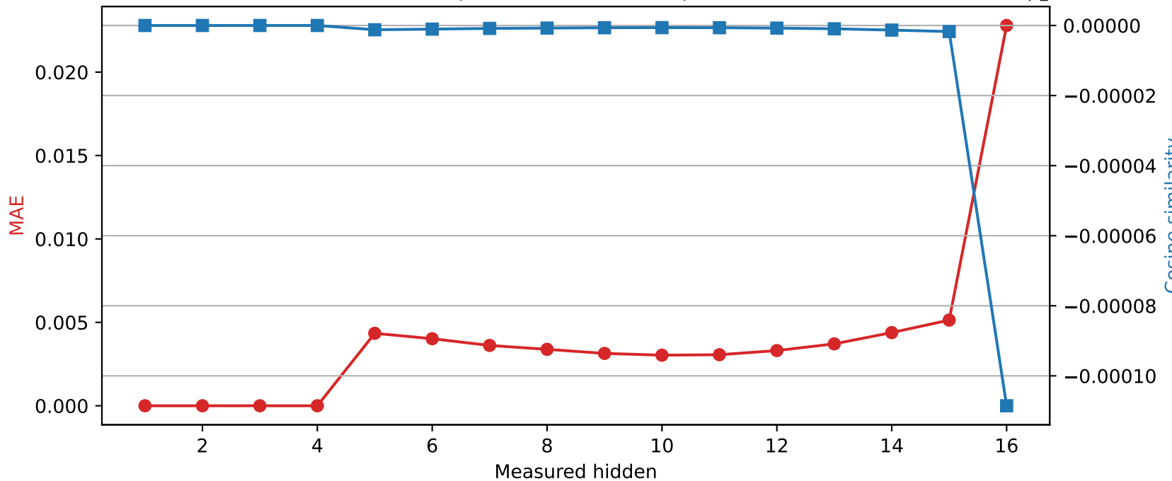
Llama-3.2-1B | Quantized layer 4 | float16 \rightarrow int8
