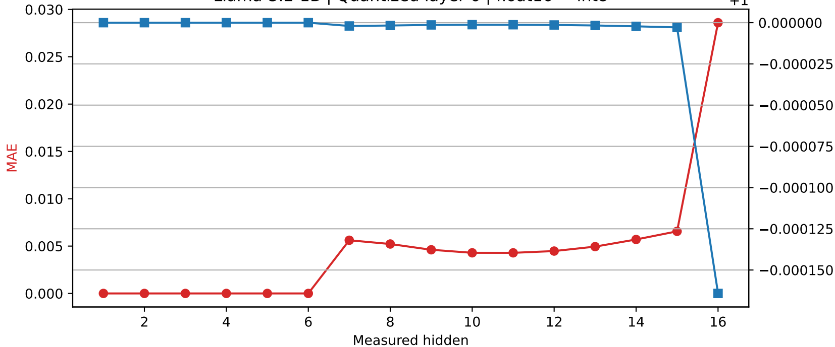
Llama-3.2-1B | Quantized layer 6 | float16 \rightarrow int8
