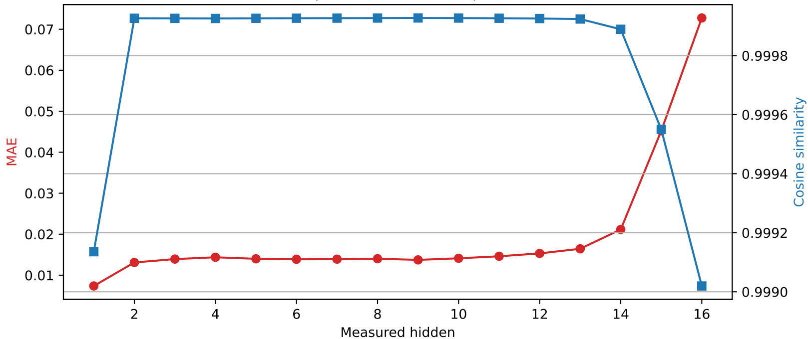
Llama-3.2-1B | Quantized layer 0 | float32 → int8
