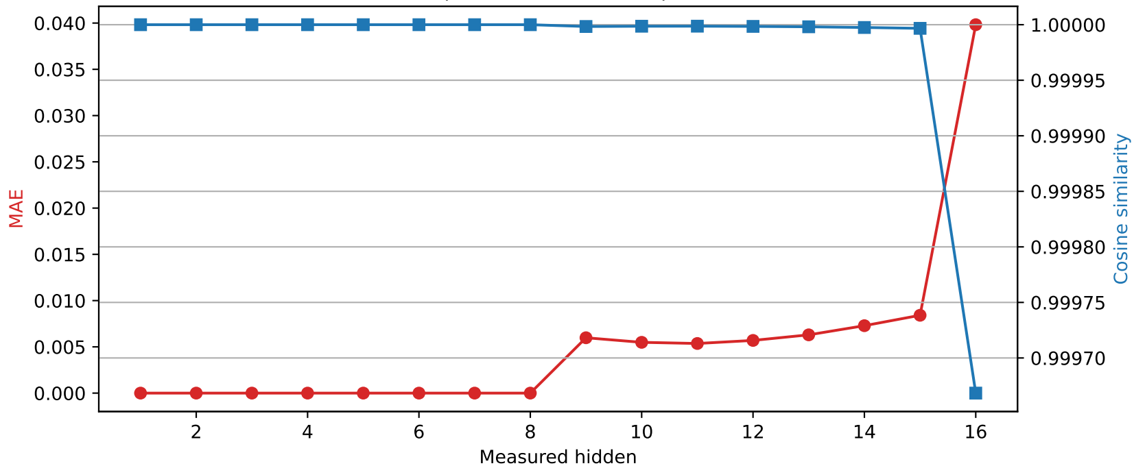
Llama-3.2-1B | Quantized layer 8 | float32 \rightarrow int8
