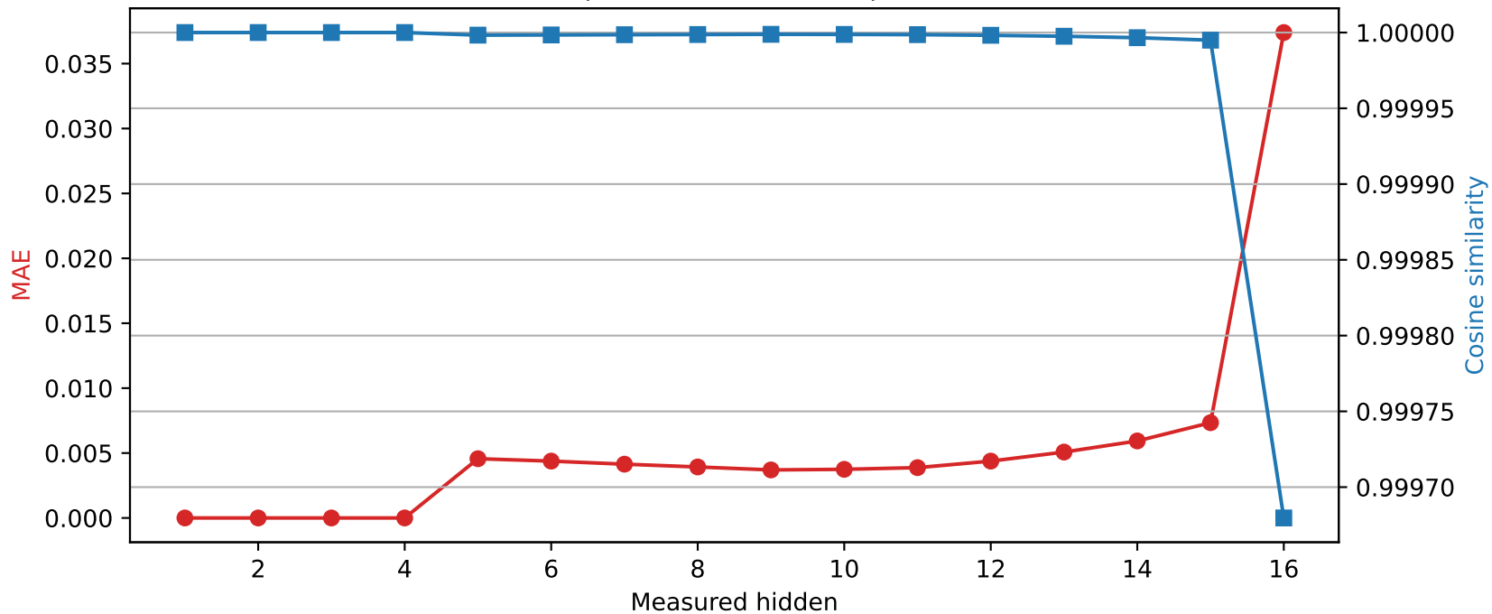
Llama-3.2-1B | Quantized layer 4 | float32 → int8
