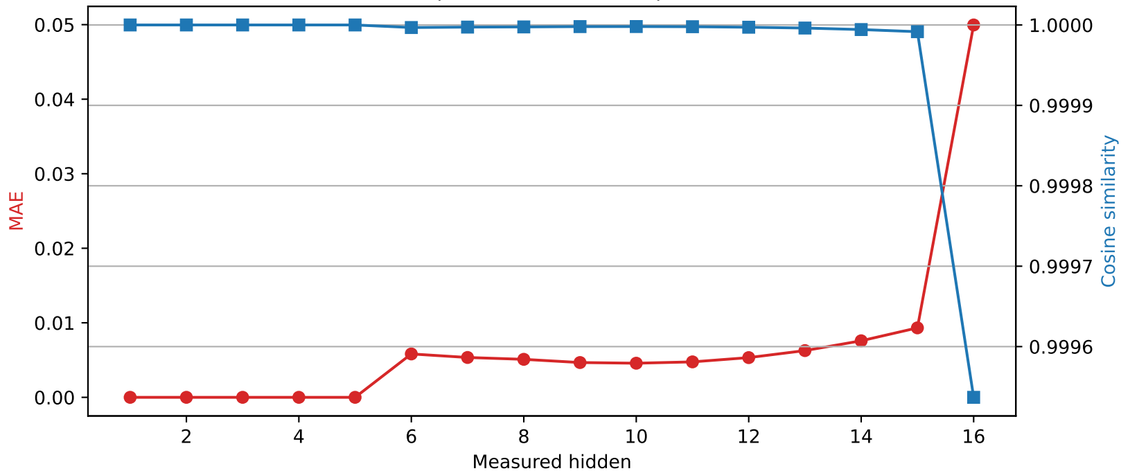
Llama-3.2-1B | Quantized layer 5 | float32 → int8
