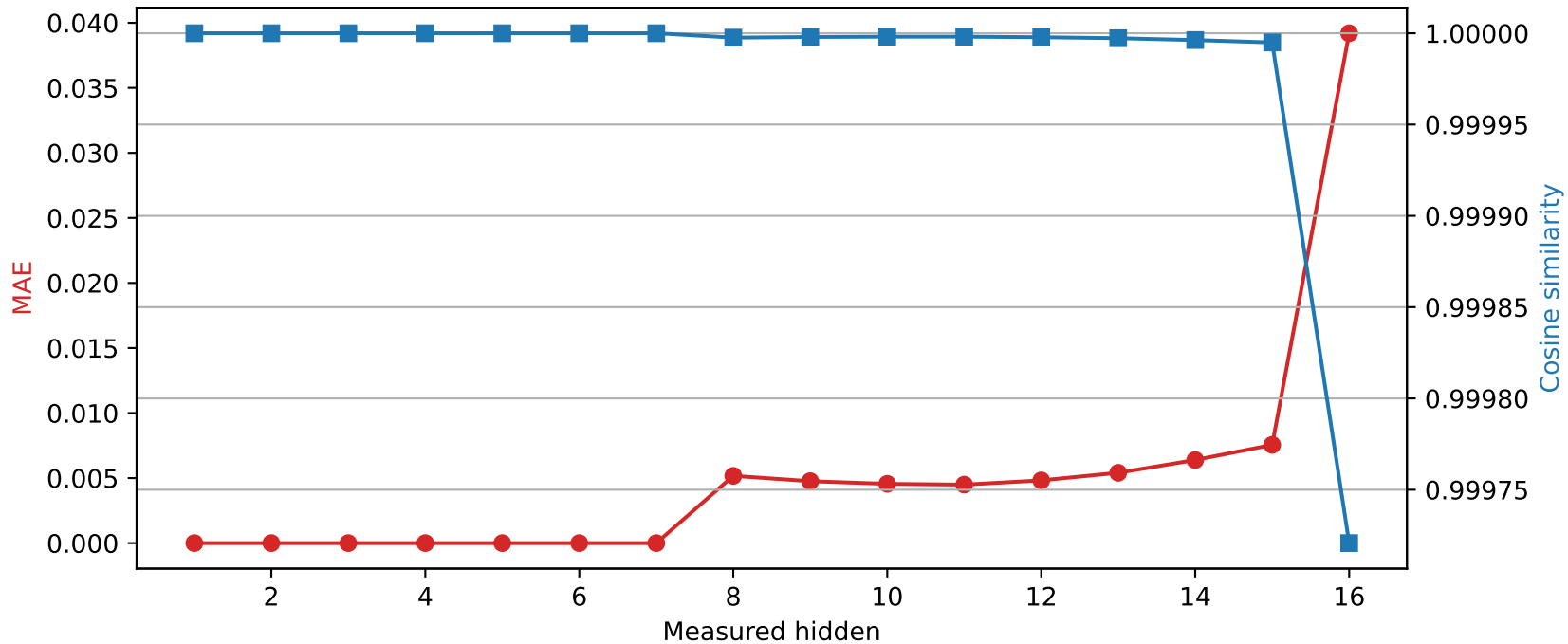
Llama-3.2-1B | Quantized layer 7 | float32 \rightarrow int8
