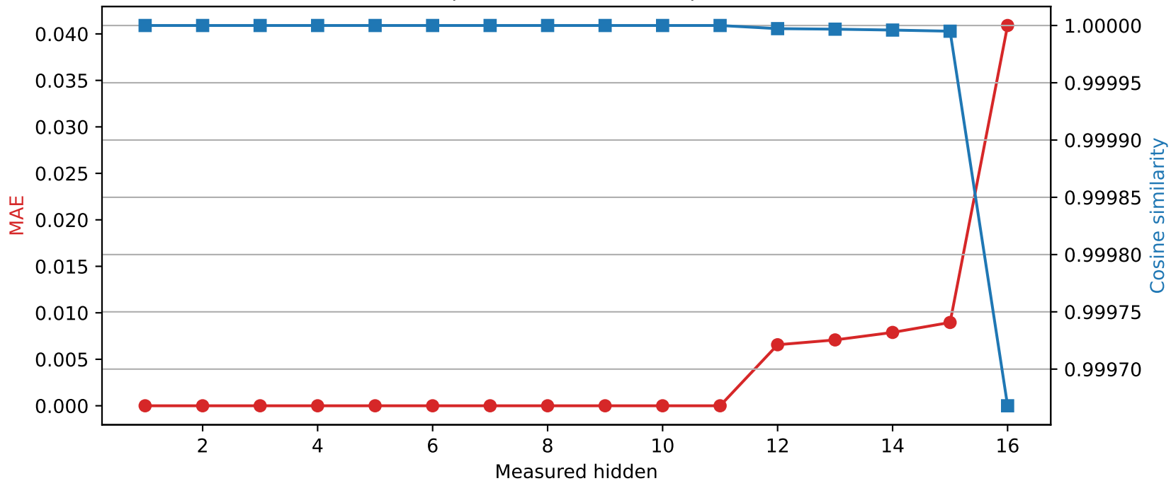
Llama-3.2-1B | Quantized layer 11 | float32 \rightarrow int8
