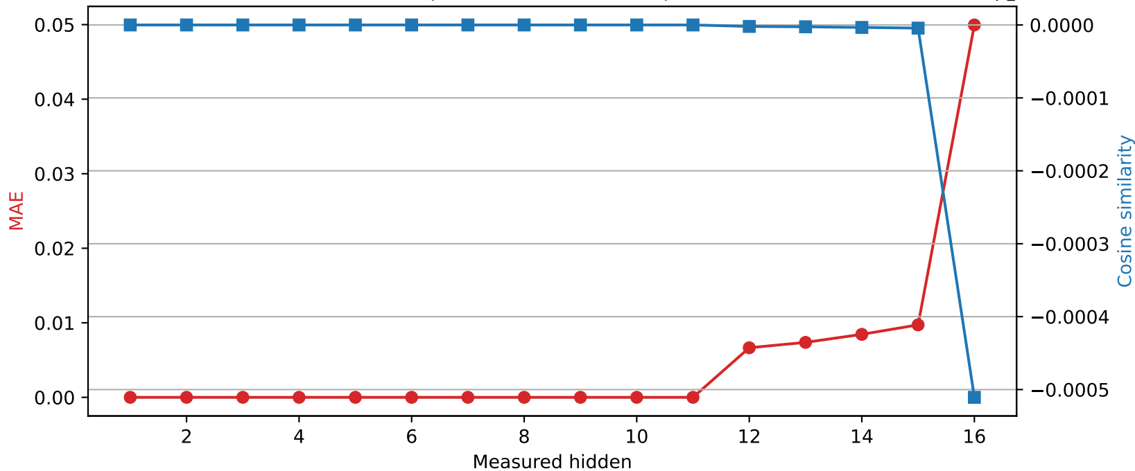
Llama-3.2-1B | Quantized layer 11 | float64 → int8
