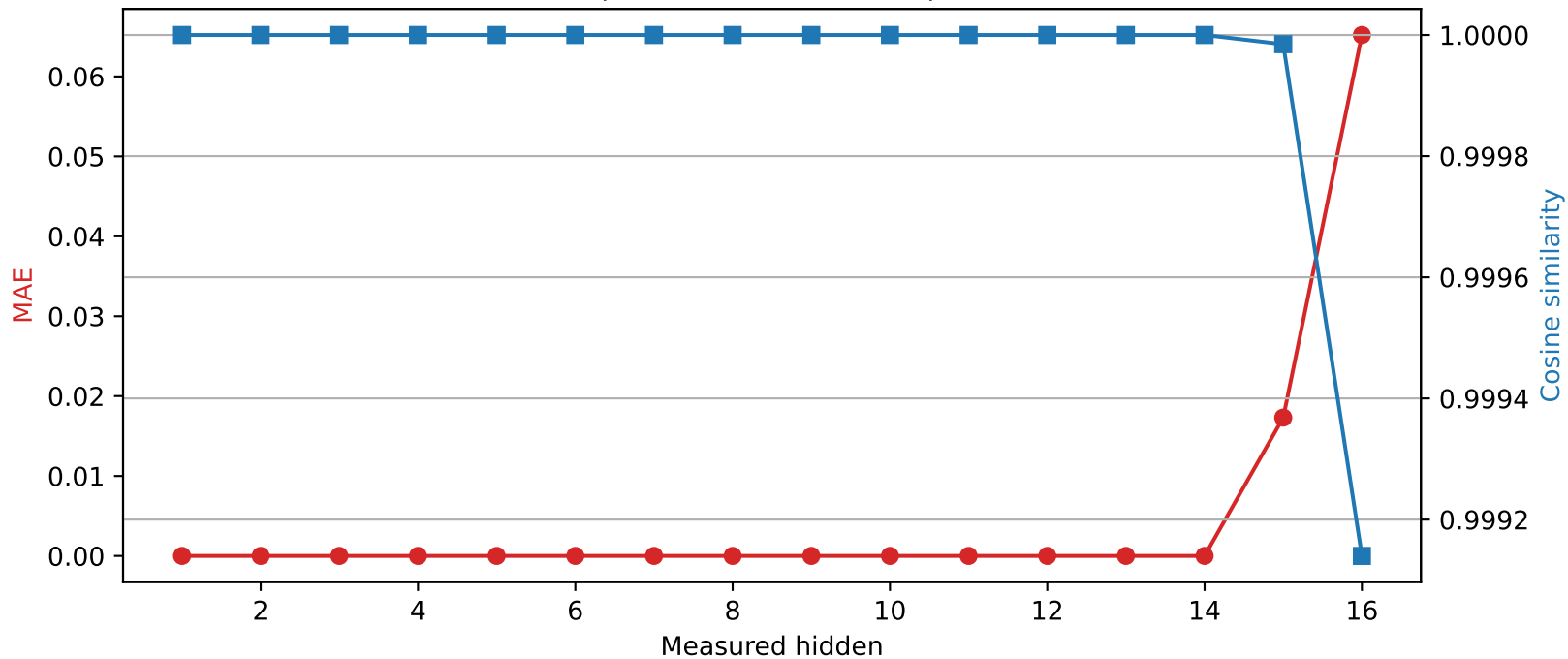
Llama-3.2-1B | Quantized layer 14 | float64 → int8
