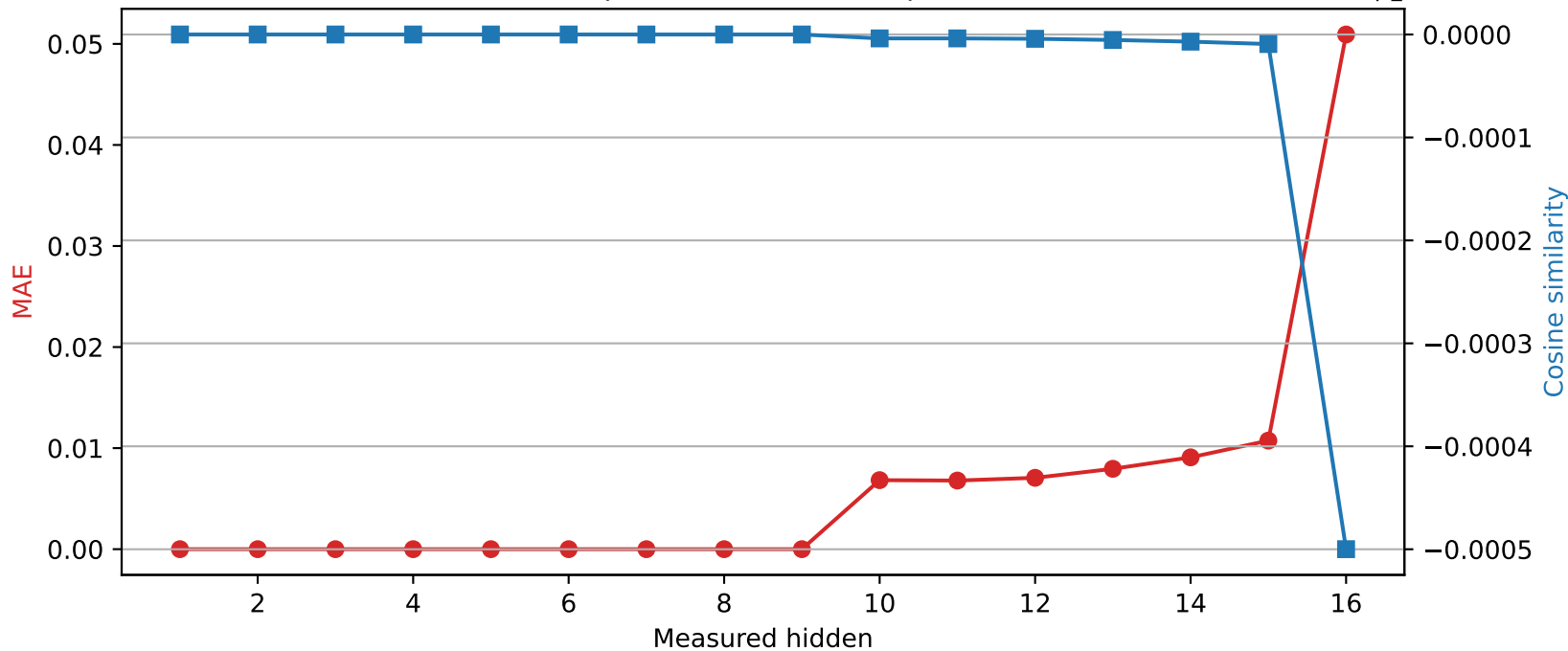
Llama-3.2-1B | Quantized layer 9 | float64 → int8
