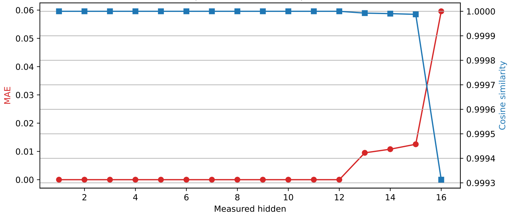
Llama-3.2-1B | Quantized layer 12 | float64 → int8
