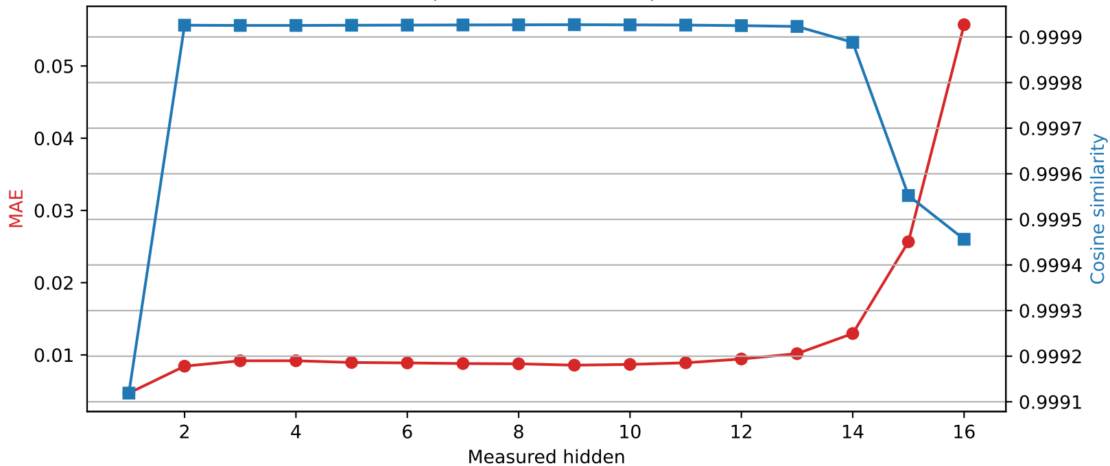
Llama-3.2-1B | Quantized layer 0 | float64 \rightarrow int8
