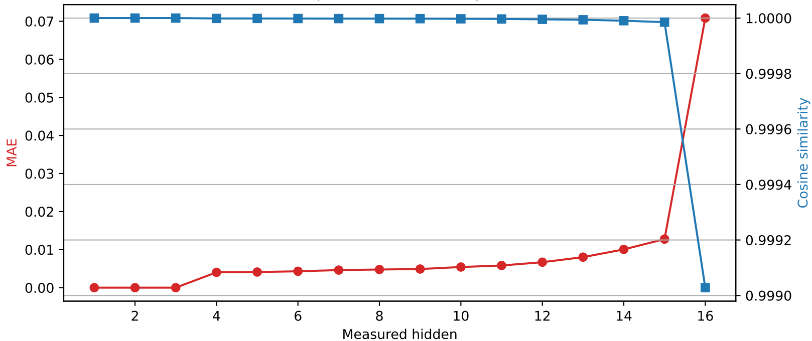
Llama-3.2-1B | Quantized layer 3 | float64 → int8
