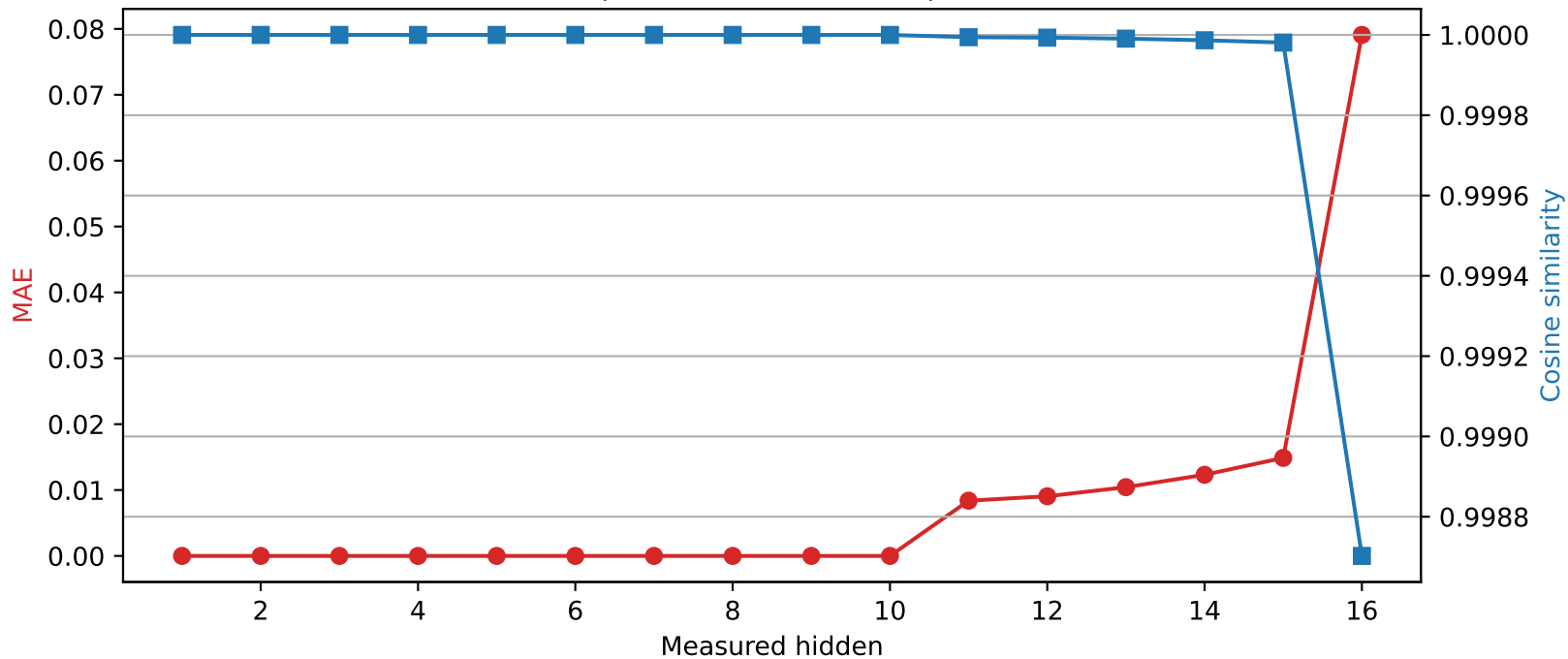
Llama-3.2-1B | Quantized layer 10 | float64 \rightarrow int8
