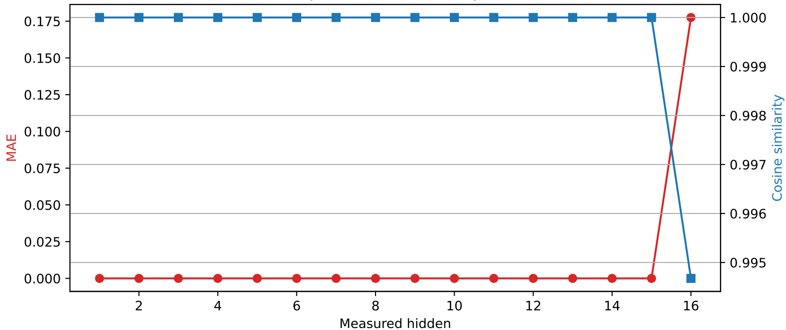
Llama-3.2-1B | Quantized layer 15 | float64 \rightarrow int8
